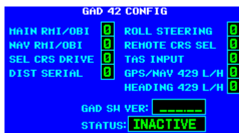
Figure 5-27. GAD 42 CONFIG Page
